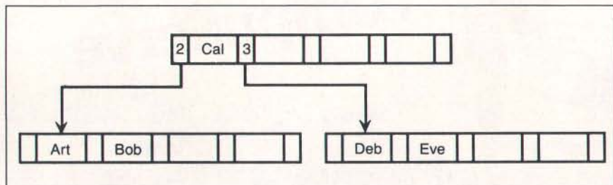
Figure 1: Reader Spear's B-tree.
